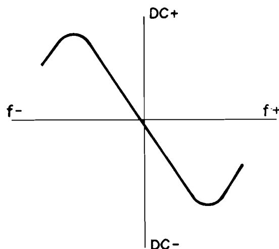
Fig. 4 Discriminator Characteristics
