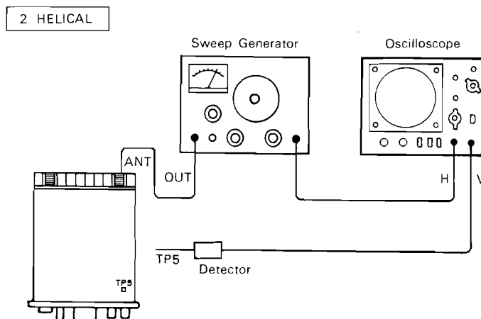
Fig. 3b. RX adjustments
