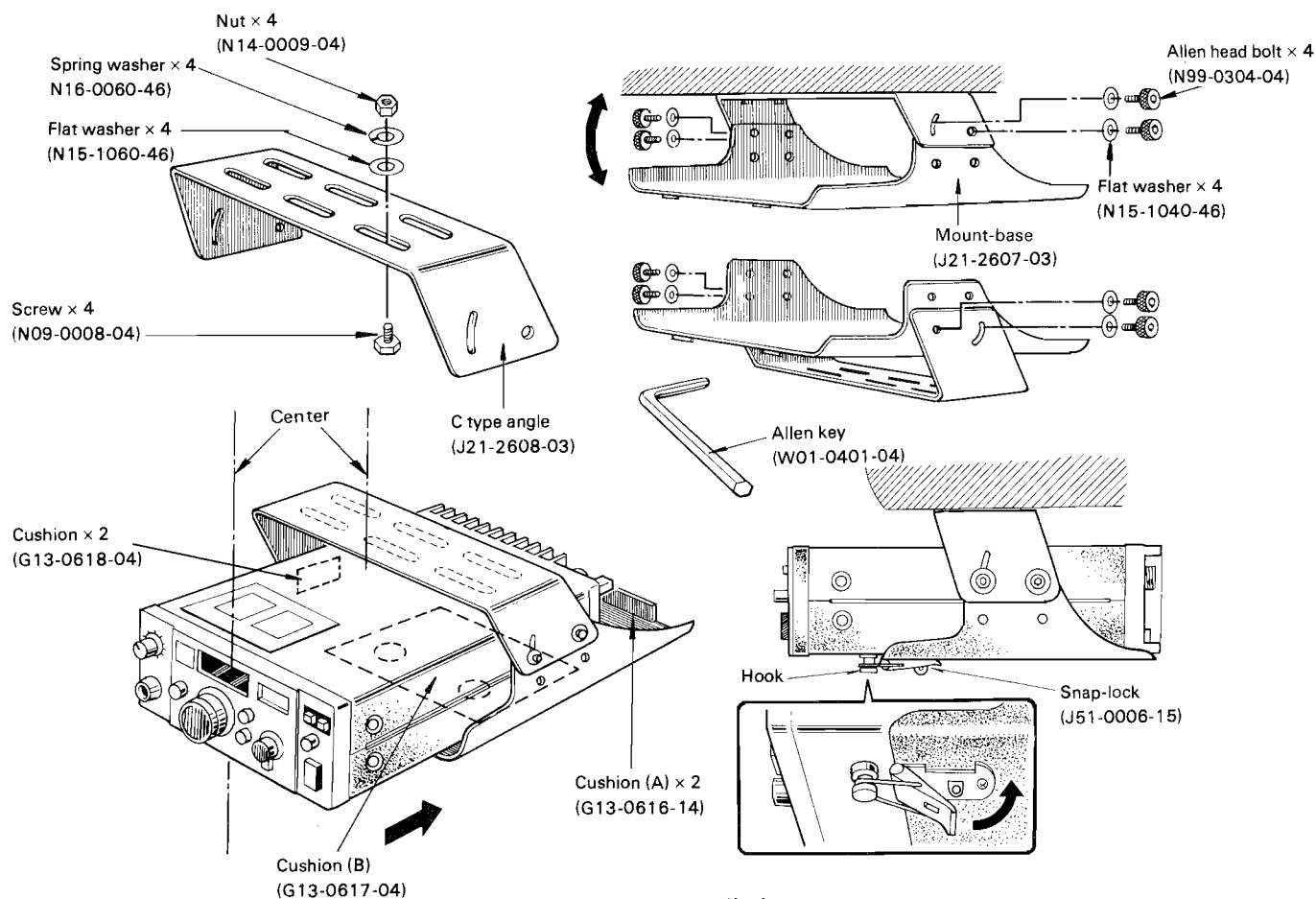
Fig. 9-2 Bracket Installation
