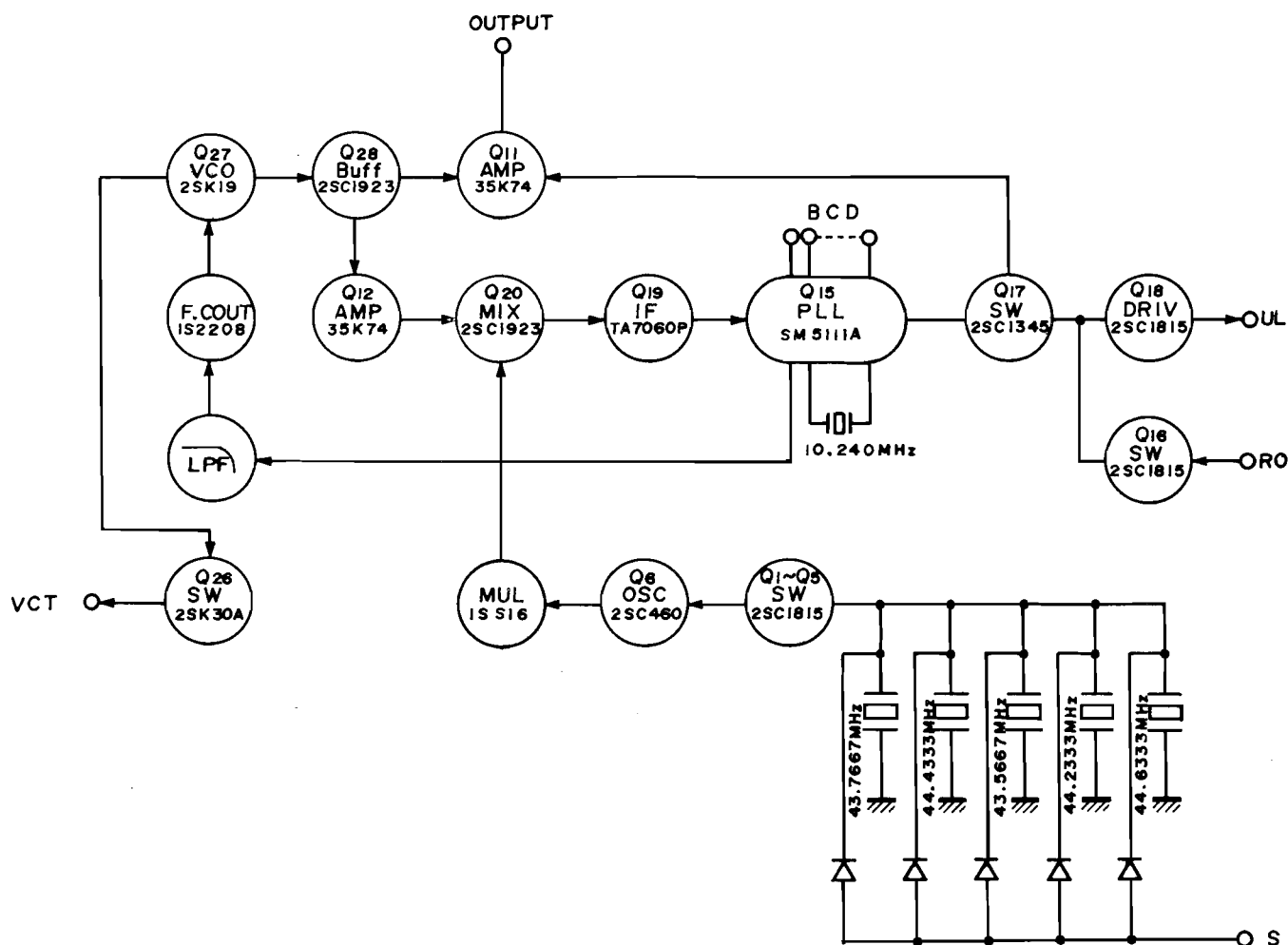
Fig. 1 PLL Circuit
