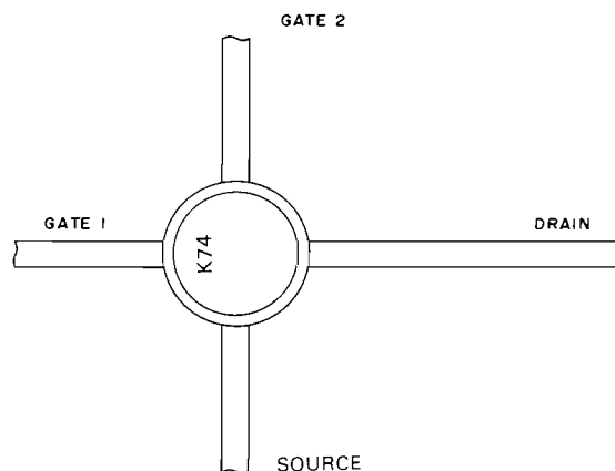
Fig. 7 3SK74 Outline
