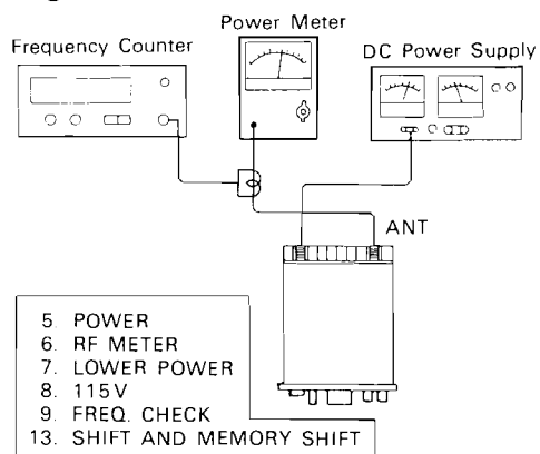
Fig. 2b. TX adjustments
