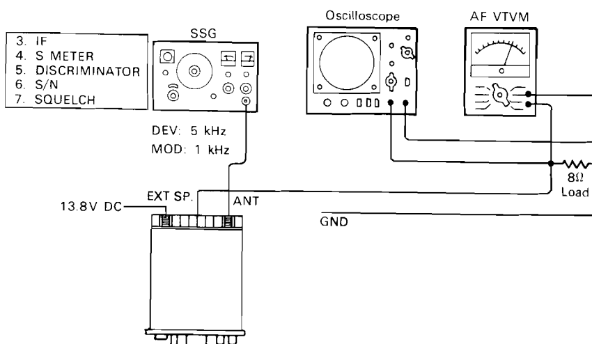
Fig. 3b. RX adjustments
