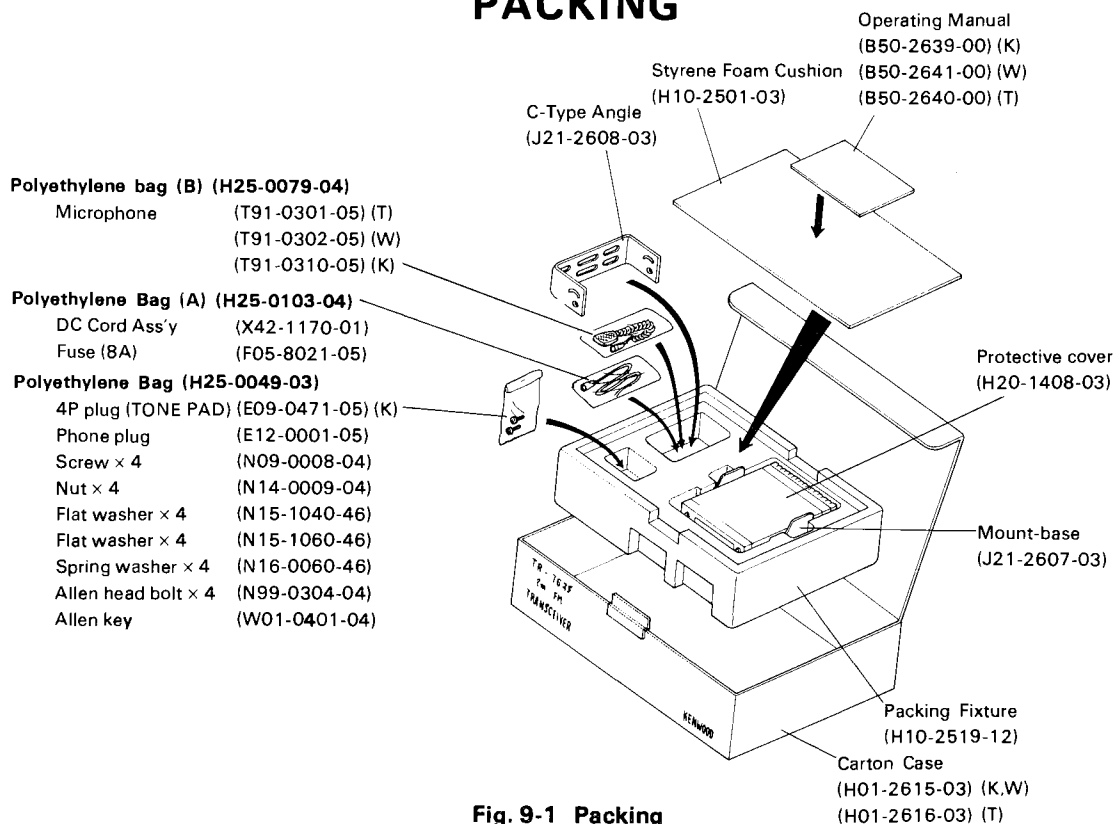
Fig. 9-1 Packing
